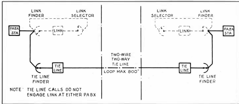
Fig. 3—Self-contained Tie Line—Function Diagram.
