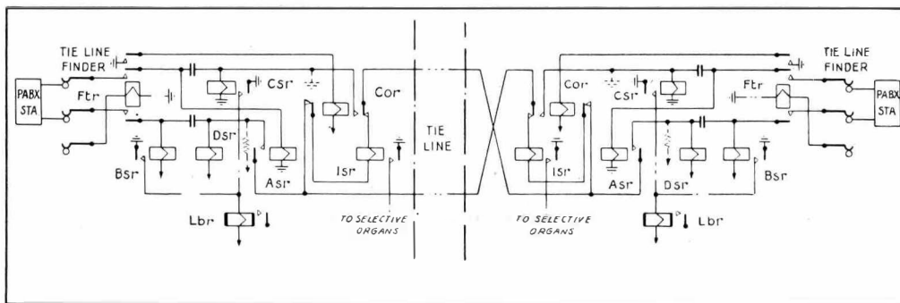
Fig. 4—Self-contained Tie Line—Switching Principle.
