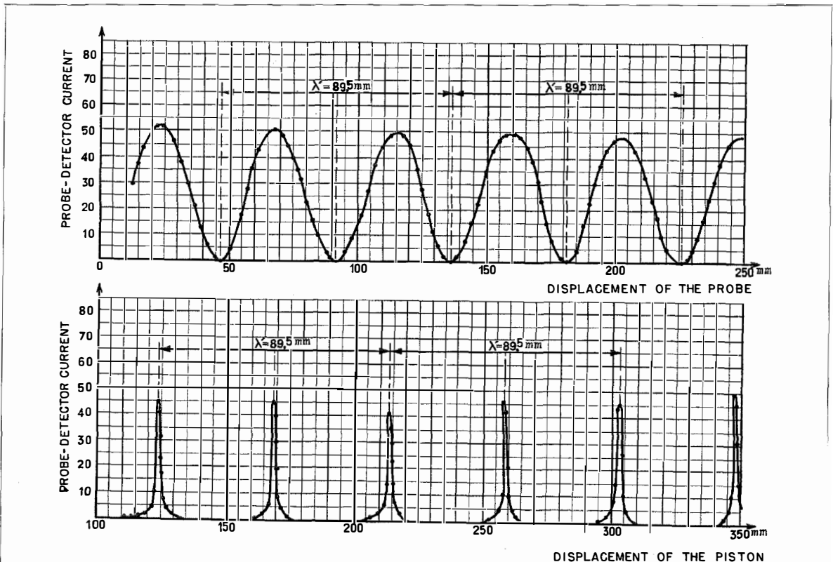
Fig. 14—Transverse Vector Distribution of an E_0 Wave along the Guide Axis (Upper Curve); and Amplitude Variation as a Function of the Resonance Chamber Length. Guide Diameter 125 mm ( \lambda = 78.5 mm).
