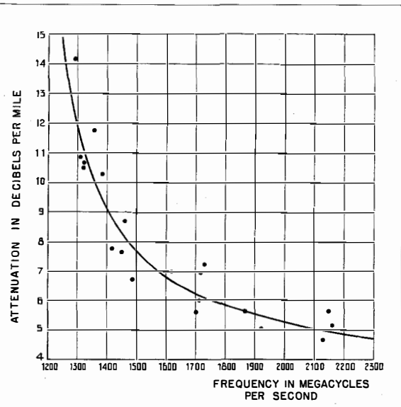
Fig. 33—Attenuation of H_1 Waves in a Copper Tube 15 cm in Diameter. The Curve is Calculated, the Dots are Experimental (Southworth's Results).
