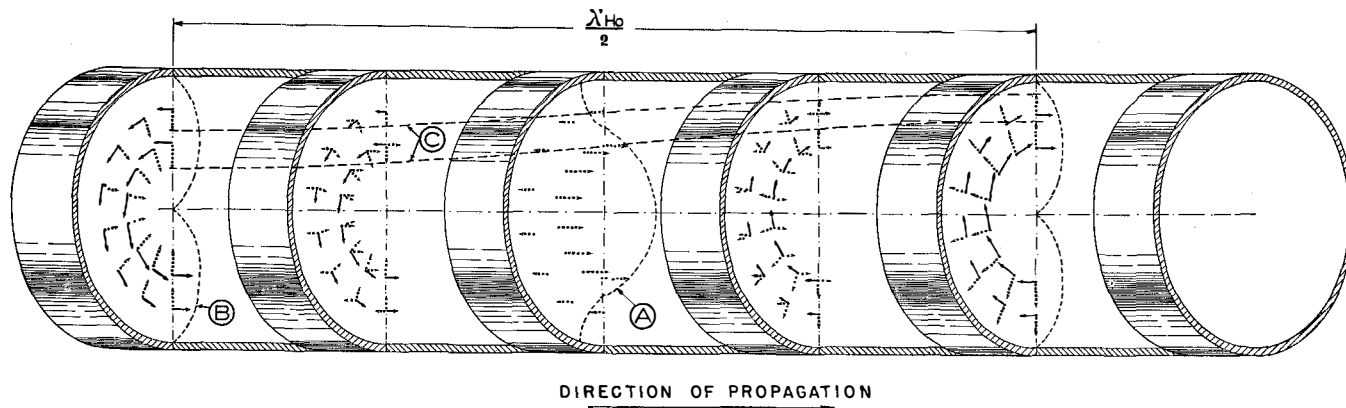
Fig. 3—Progressive H_0 Wave : Electric (full lines) and Magnetic (dotted lines) Vectors. Curve A : distribution of longitudinal vectors along the radius (Bessel function J_0(K\rho) ). Curve B : distribution of transverse vectors along the radius (Bessel function J_1(K\rho) ). Curve C : distribution of all vectors along the axis (sinusoidal function).
