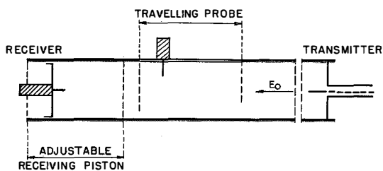
Fig. 16—Schematic of a Transmitter and Receiver ( E_0 Wave). The Detector Reveals the Presence of an H_1 (Parasitic) Wave.
