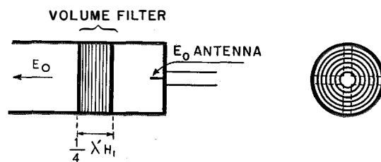
Fig. 17—Schematic of a Filter for Purifying E_0 Waves.
