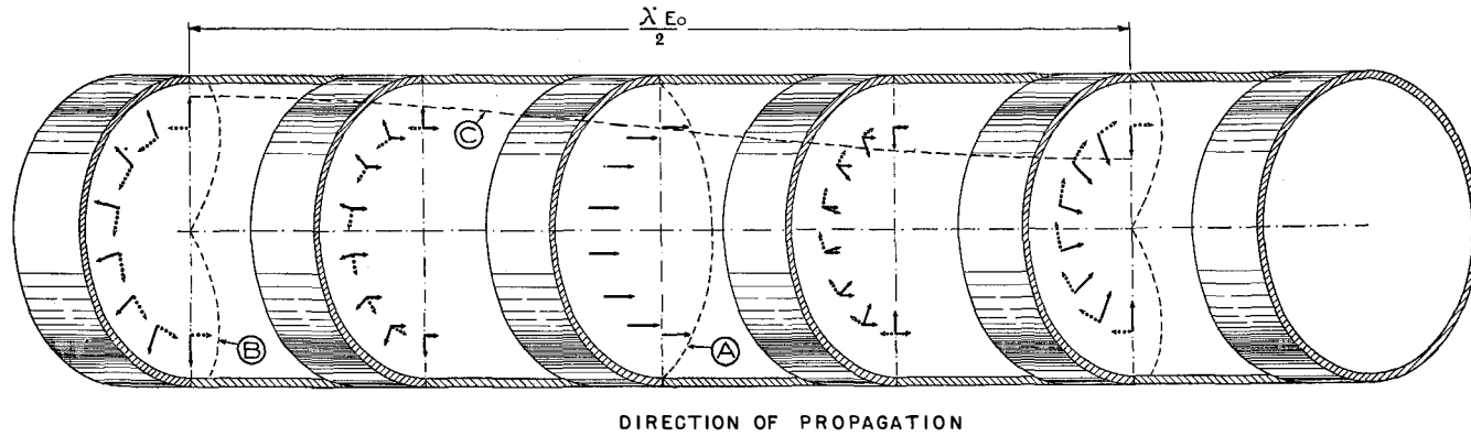
Fig. 2—Progressive E_0 Wave : Electric (full lines) and Magnetic (dotted lines) Vectors. Curve A : distribution of longitudinal vectors along the radius (Bessel function J_0(K\rho) ). Curve B : distribution of transverse vectors along the radius (Bessel function J_1(K\rho) ). Curve C : distribution of all vectors along the axis (sinusoidal function).
