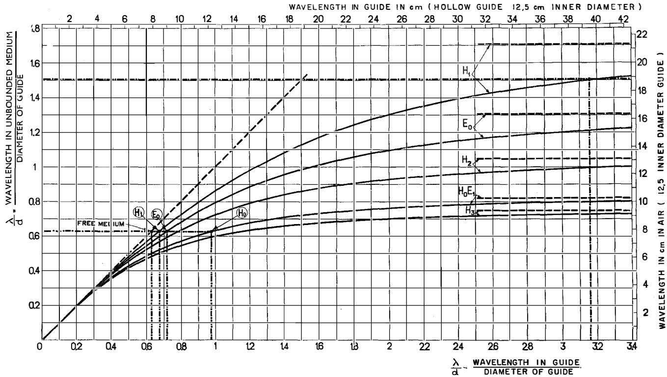
Plate II—Determination of Wavelengths in a Guide. Wavelengths in Free Medium and in the Guide are Plotted relatively to the Guide Diameter.
