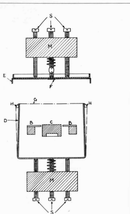
Fig. 4—Diagram to show the electrode construction. BB, shield round cathode; C, indirectly heated nickel cathode; D, steel frame of grid; E, outer "guard" part of the anode; F, centre section of the anode, area 0.575 sq. cm insulated from E by heater coating; G, molybdenum grid laterals; HH, screwed rods fixing the grid pitch; MM, supporting frames; SS, adjusting screws.
