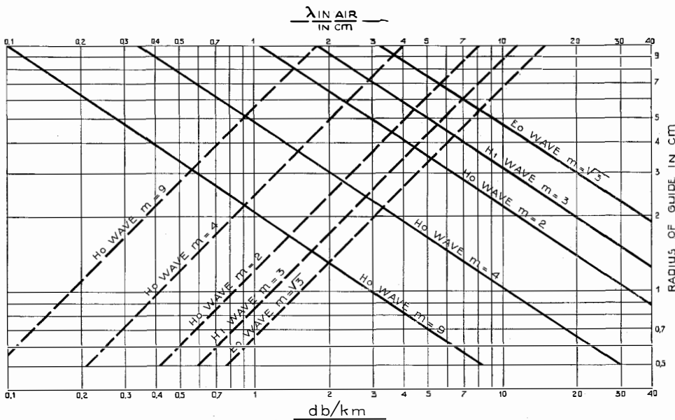
Plate III—Optimum Operating Wavelengths of Different Types Versus Guide Radius (broken lines), and Corresponding Attenuation due to Copper Loss (full lines).
